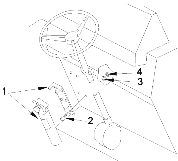
FIRE EXTINGUISHER IN DRIVER COMPARTMENT
